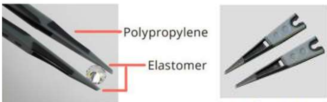
Replacement tip (401-063)
