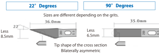
Thin Diamond File Tip 22°
